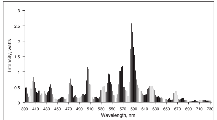
Figure 26. Metalarc MP clear 400-watt lamp.
