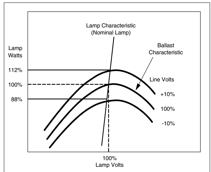
Figure 16. Typical output regulation reactor ballast (LAG).
