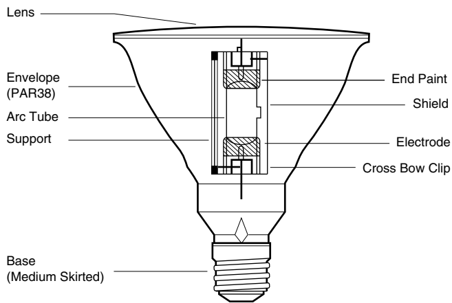
Figure 8. Construction of a PAR38 Metalarc Pro-Tech Lamp.
