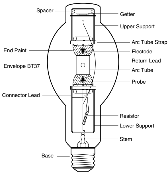
Figure 2. Construction of 400-watt Universal-Burning Metalarc Lamp.
