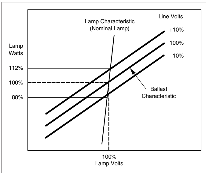
Figure 17. Typical output regulation autotransformer (CWA) ballast.
