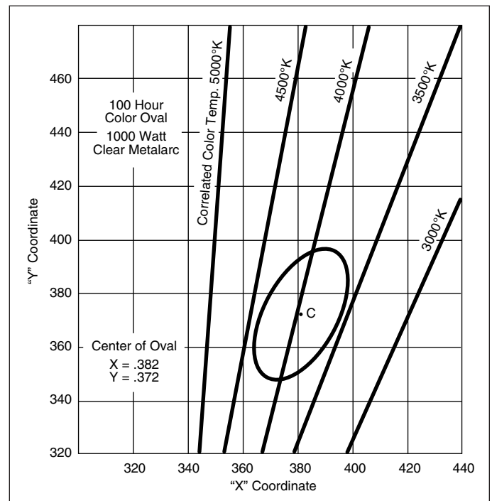
Figure 22. Typical Chromaticity Diagram.
