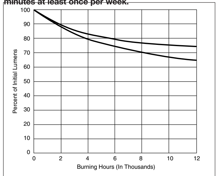
Figure 14. Typical lumen maintenance curve.
