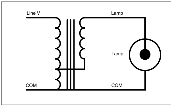
Figure 19. Typical high reactance autotransformer circuit without capacitor.
