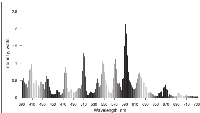
Figure 29. Super Metalarc coated 400-watt lamp.
