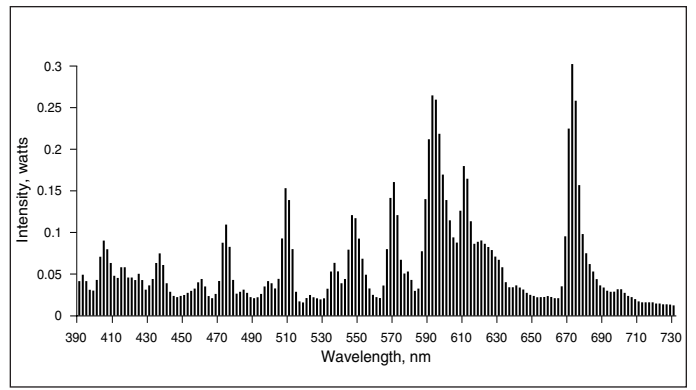
Figure 24. Metalarc diffuse coat 100-watt lamp.
