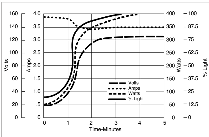
Figure 21. Warm-up characteristics of a 400-watt Metalarc Lamp.
