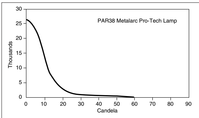
Figure 9. Typical Candlepower Distribution Curve (70W).
