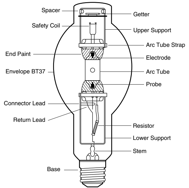
Figure 6. Construction of a Metalarc Safeline Lamp.
