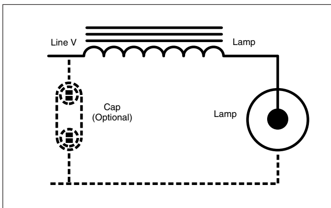
Figure 18. Typical reactor circuit with optional capacitor.
