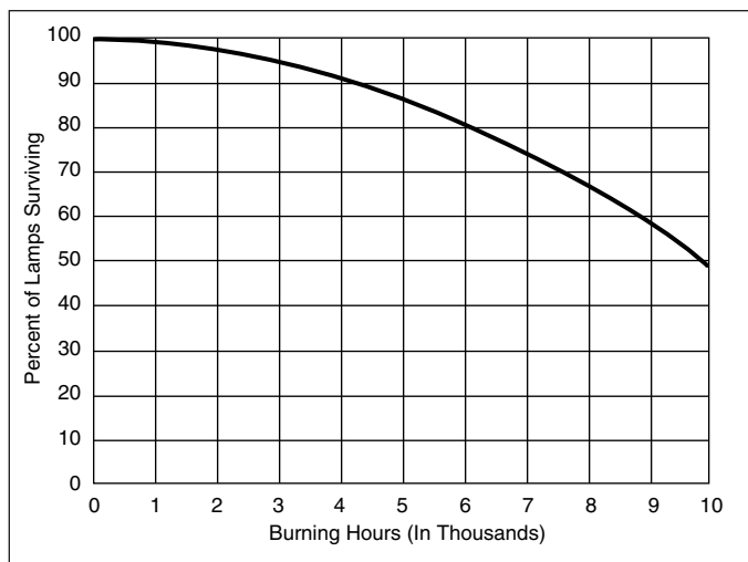
Figure 15. Typical lamp mortality curve.
