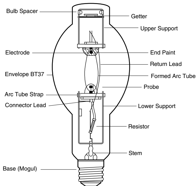
Figure 4. Construction of a vertical Super Metalarc Lamp.
