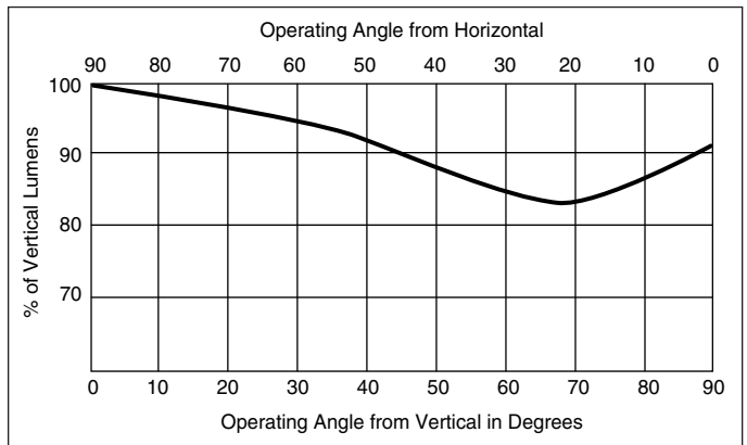
Figure 10. Metalarc Lamp light output versus lamp operating position.
