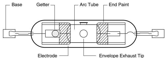
Figure 7. Construction of a Brite-Line Lamp.
