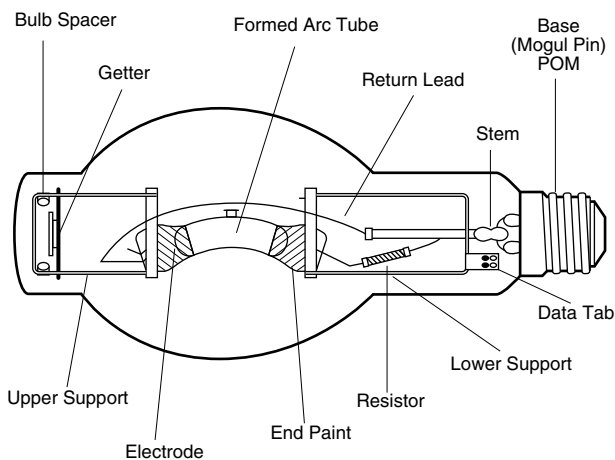
Figure 3. Construction of a horizontal Super Metalarc Lamp.
