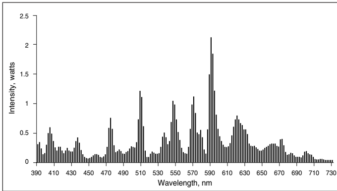
Figure 25. Metalarc coated 3K 400-watt lamp.
