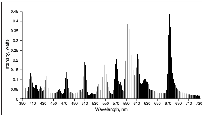
Figure 23. Metalarc clear 100-watt lamp.
