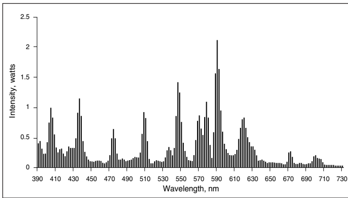
Figure 27. Metalarc coated 400-watt lamp.
