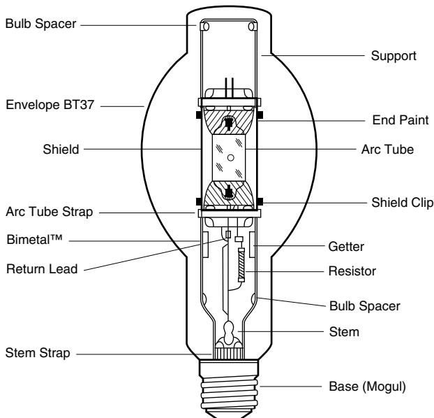
Figure 5. Construction of a Metalarc Pro-Tech Lamp.
