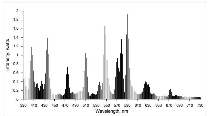
Figure 28. Metalarc clear 400-watt lamp.
