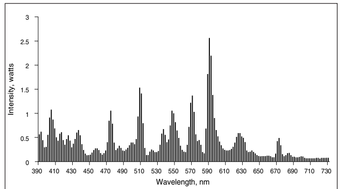
Figure 30. Super Metalarc clear 400-watt lamp.
