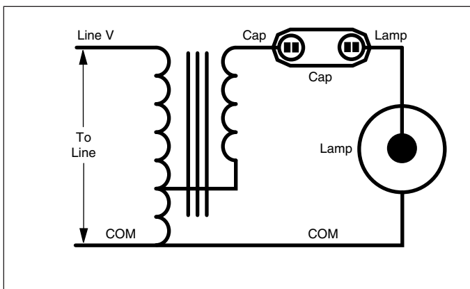
Figure 20. Typical constant wattage autotransformer circuit.
