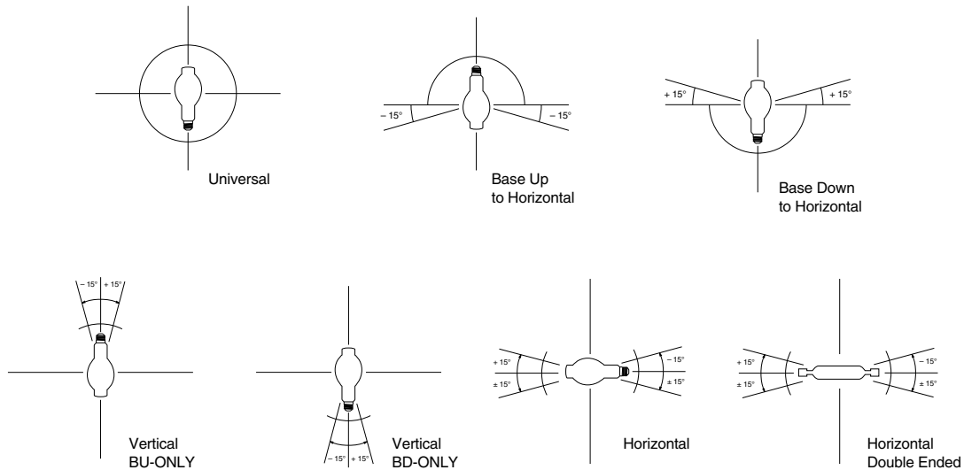
Figure 13. Operating position guide.
